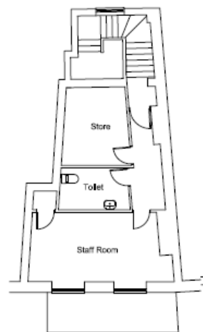
Existing First Floor Plan (SCALE 1:50)
