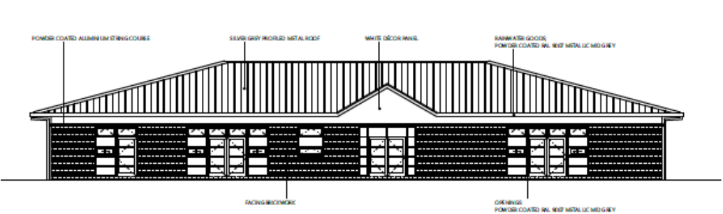
EAST ELEVATION
