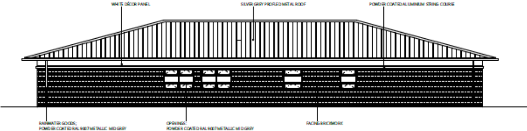
WEST ELEVATION
