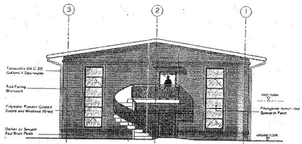
OFFICE GABLE ELEVATION
