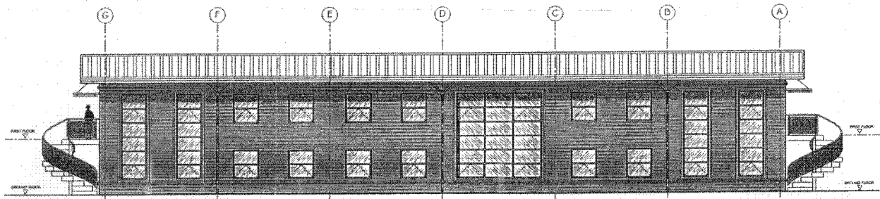
TYPICAL CANAL ELEVATION
