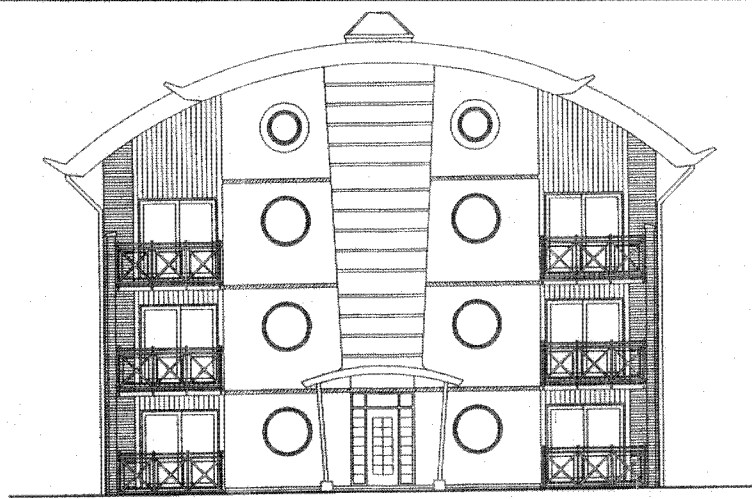
FRONT / REAR ELEVATION - 12 UNIT BLOCK
