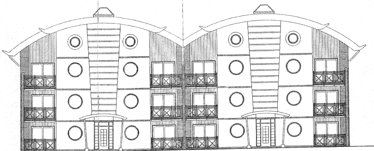
FRONT / REAR ELEVATION - 24 UNIT TERRACE
