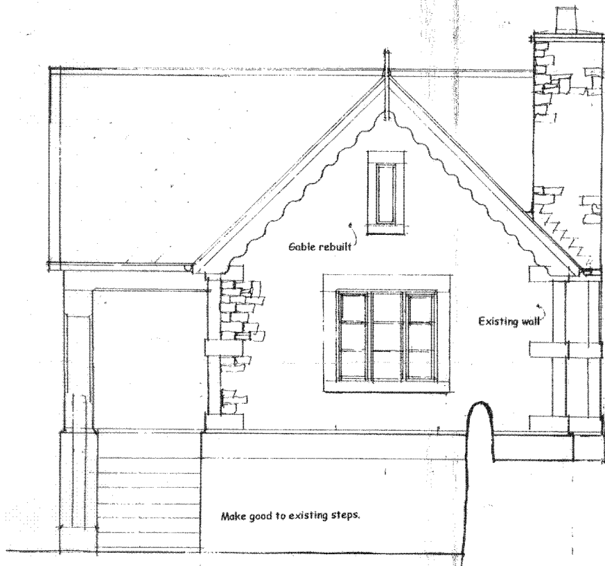
South Elevation
