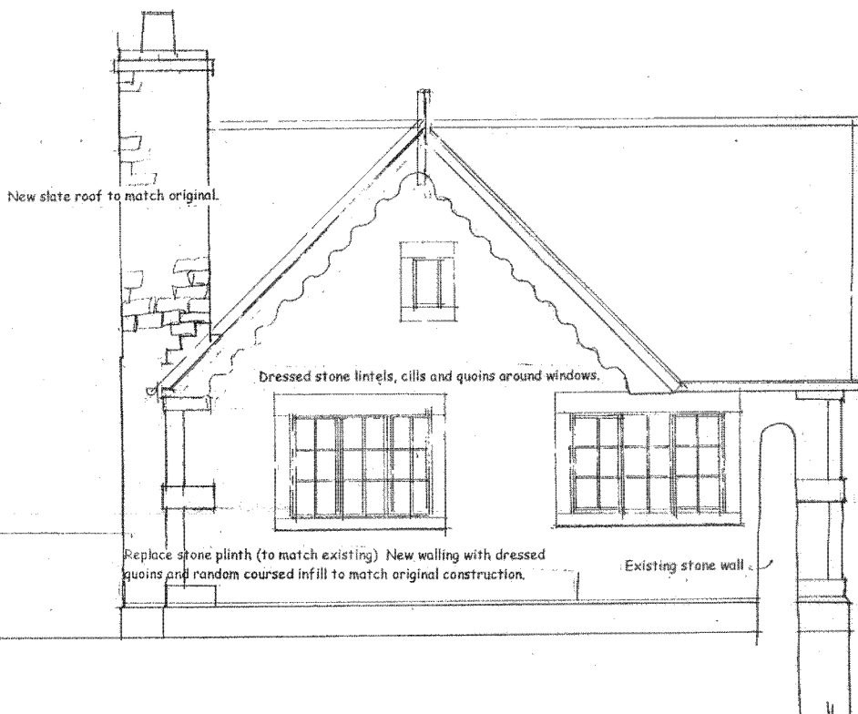
North Elevation
